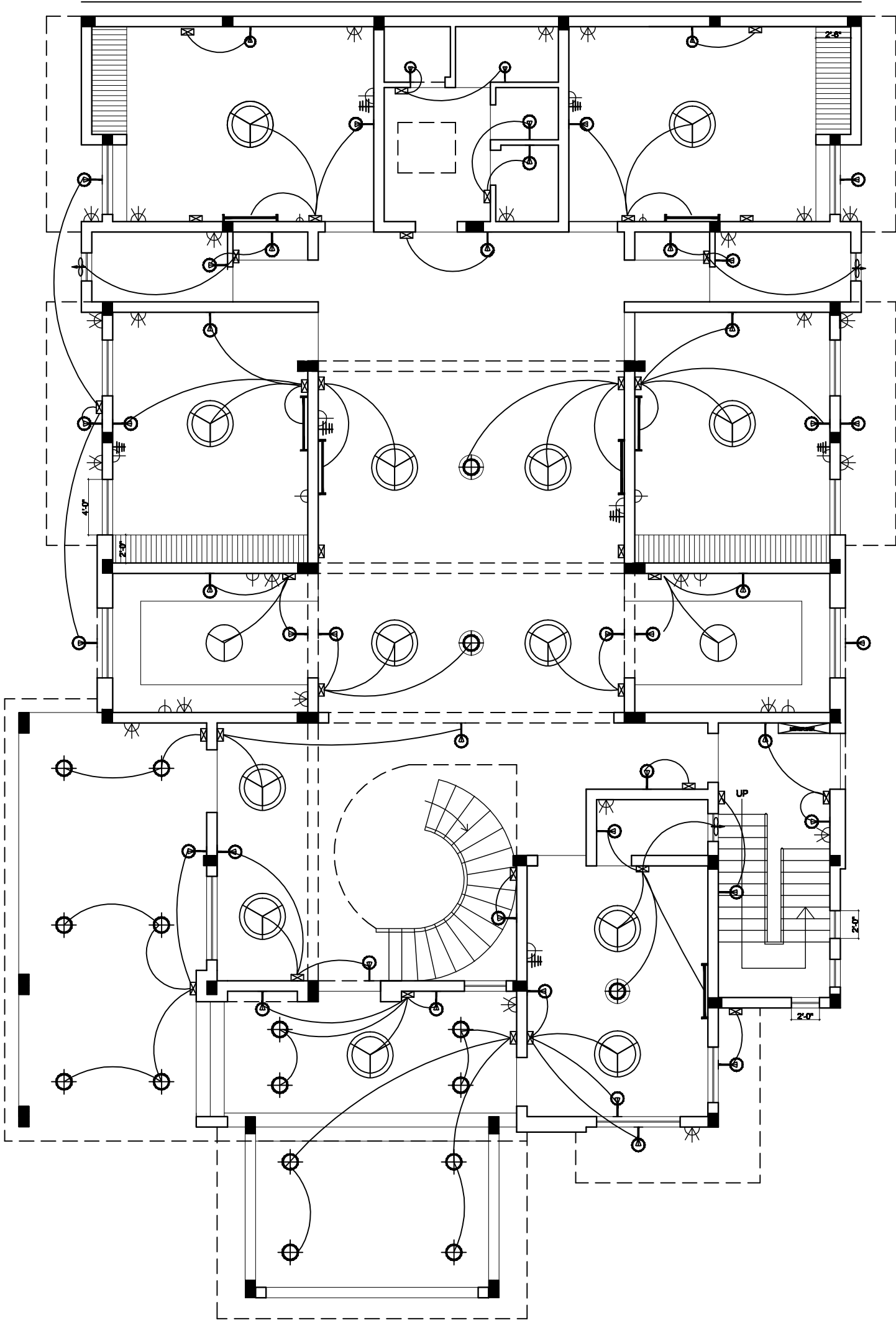
ELECTRICAL PLAN
